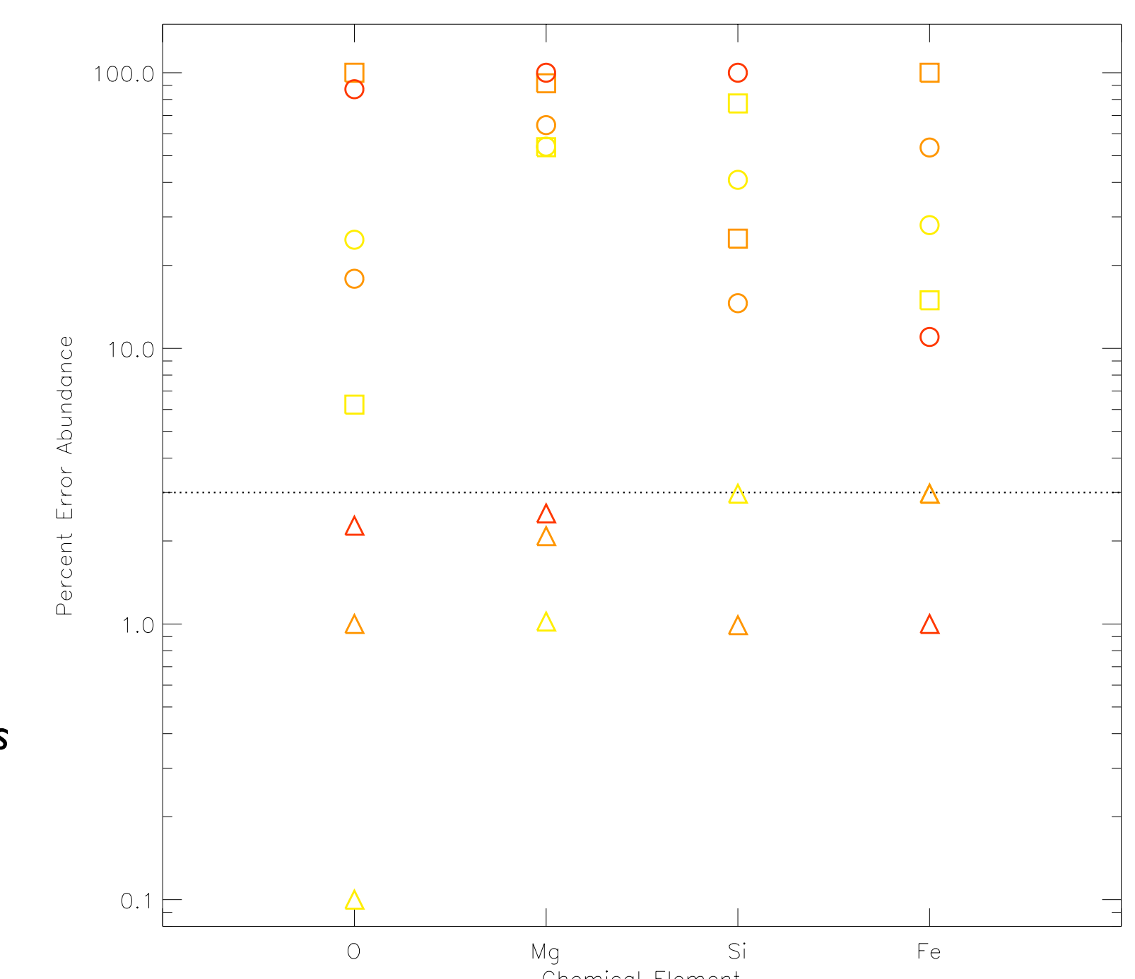
Fig. 4. Percent errors in abundance measurements of silicate grain-forming elements assuming abundances from Wilms et al. (2001), in spectra from Chandra ACIS-S, LEG (circles), XMM-Newton RGS (squares) and IXO Ucal (triangles) when N_H is 5 \times 10^{21} \text{ cm}^{-2} (yellow), 5 \times 10^{22} \text{ cm}^{-2} (orange), and 5 \times 10^{23} \text{ cm}^{-2} (red). Exposure times were 50 ks for Chandra and XMM, and 20 ks for IXO. The dotted line indicates 3% error.
