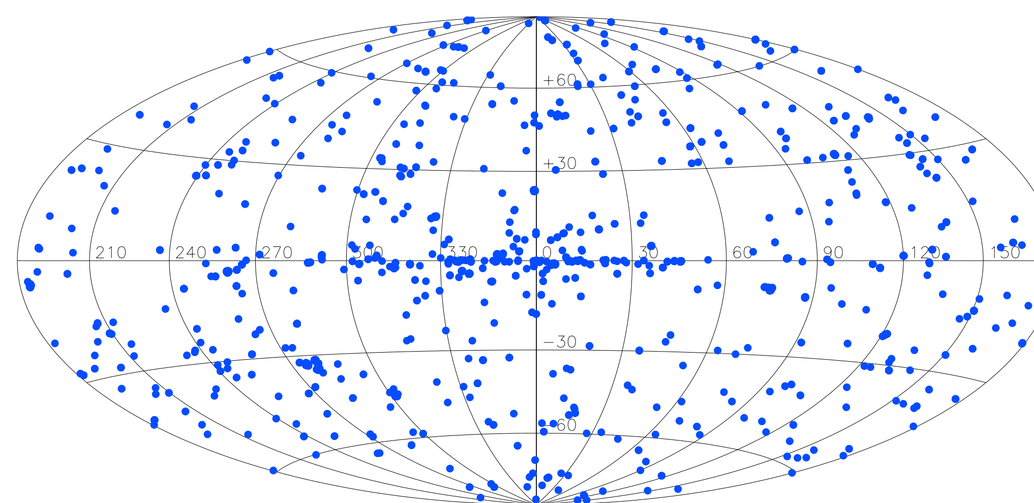
Fig. 3. Sightlines for which IXO will be able to determine abundances of silicate-forming elements to better than 20%.
