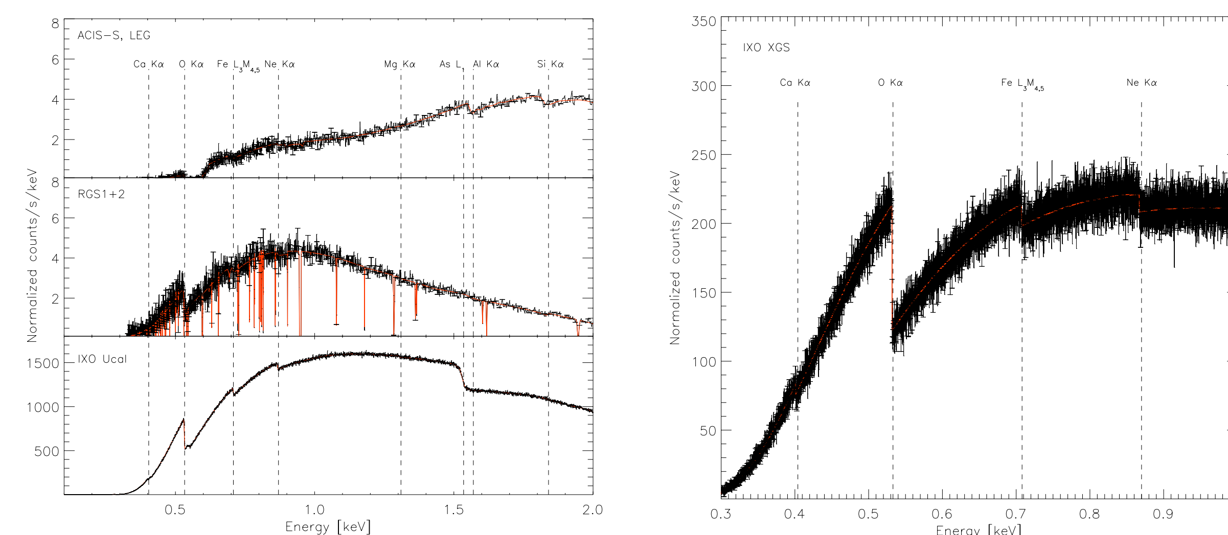
Fig. 2. Comparison of the modeled spectrum of X Per obtained with different X-ray observatories. Left: Top: Chandra ACIS-S, LEG ( t = 50 \text{ ks} ); Middle: XMM-Newton RGS ( t = 50 \text{ ks} ); Bottom: IXO Ucal ( t = 20 \text{ ks} ). Right: IXO XGS ( t = 50 \text{ ks} ).
